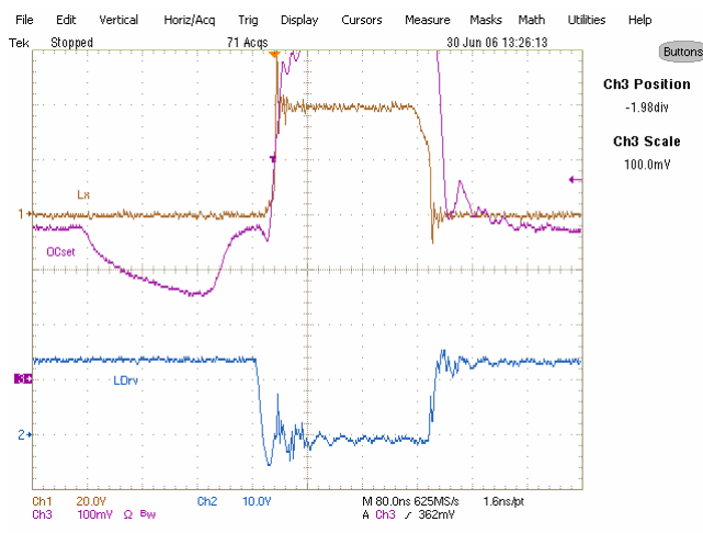
Fig. 8: OCset pin during normal condition Ch1: Inductor point, Ch2:Ldrv, Ch3:OCSet
