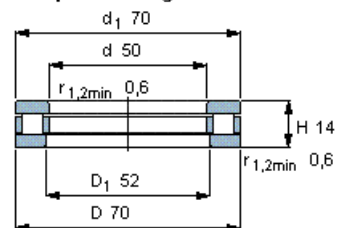
Complete bearing
