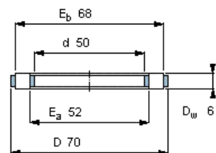
Roller and cage thrust assembly
