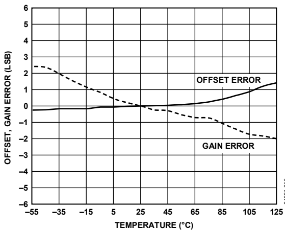
Figure 19. Offset and Gain Error vs. Temperature
