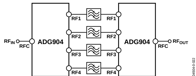
Figure 28. Filter Selection
