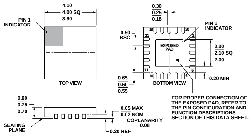
Figure 32. 20-Lead Lead Frame Chip Scale Package [LFCSP_WQ] 4 mm × 4 mm Body, Very Very Thin Quad (CP-20-6)
