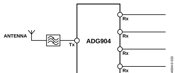
Figure 29. Tx/Rx Switching
