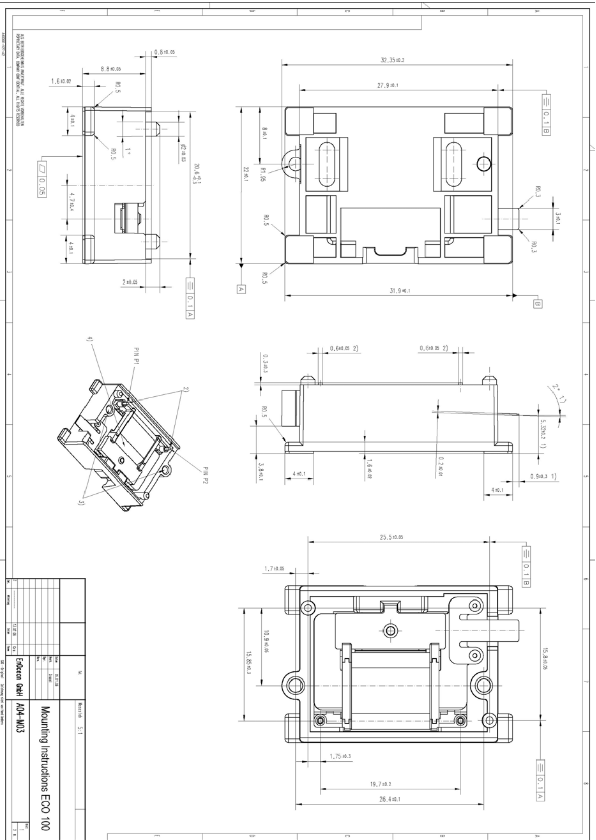
Figure 2: Mechanical dimensions
