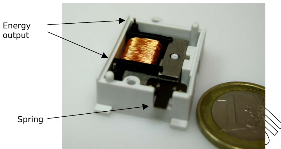
Figure 1: Electro-dynamic energy harvester ECO 100
