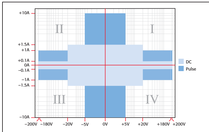
Models 2611A and 2612A I-V capability
