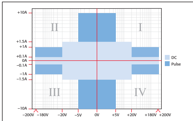
Models 2635A and 2636A I-V capability
