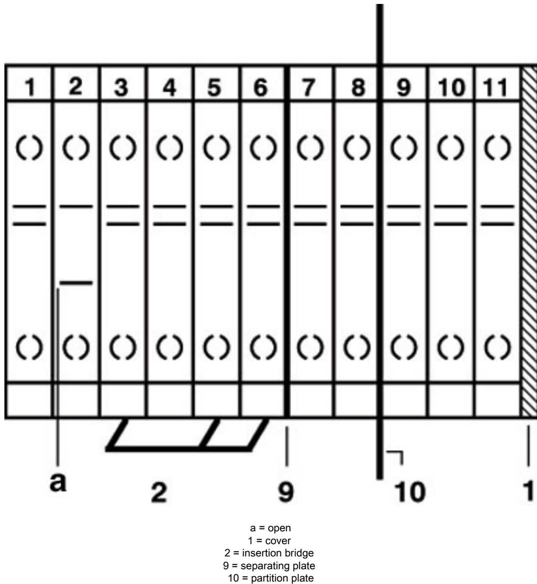
Circuit diagram
