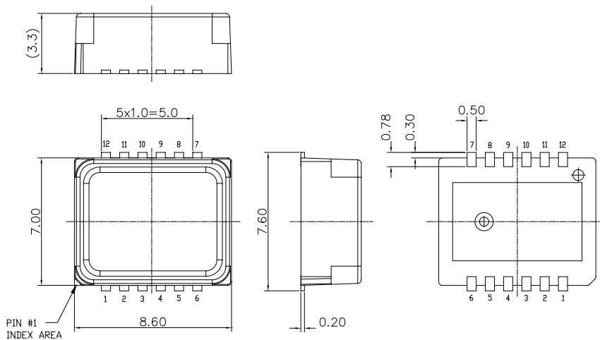
Figure 2. Housing dimensions
