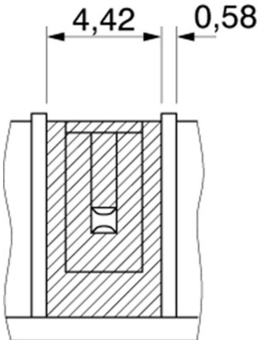
Dimensioned drawing
