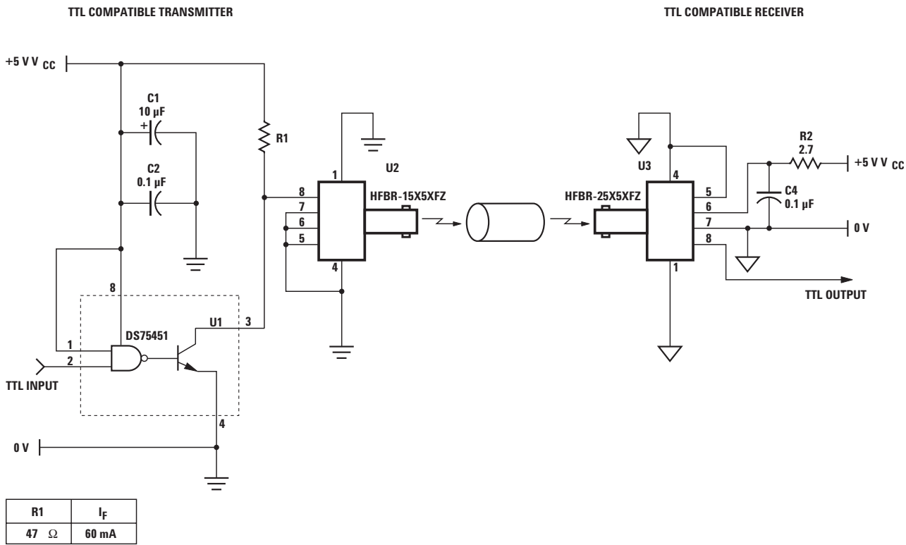
Figure 4. Recommended transmitter and receiver drive circuit (I F, on = 60 mA nominal at T A = 25°C)
