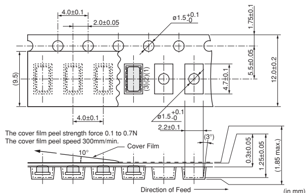
CSTCR_G_B
