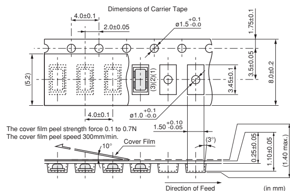
CSTCE_V13L/CSTCE_VH3L
