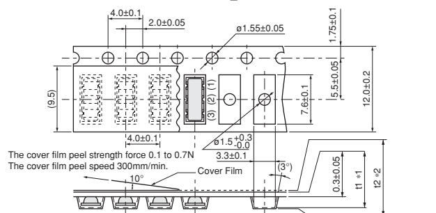
CSTCC_G
