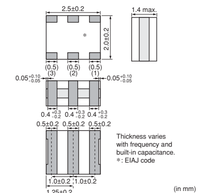
CSTCW_X 20.01-70.00MHz
