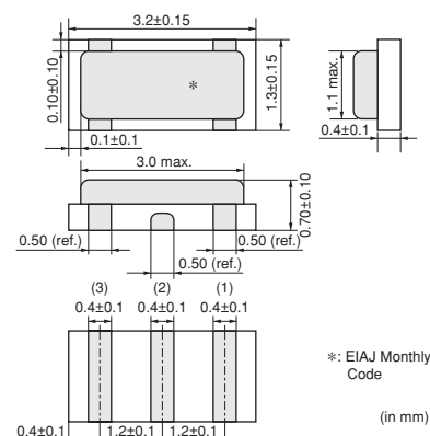
CSTCE_G15L/CSTCE_GH5L 8.00-13.99MHz
