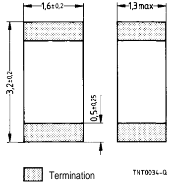
Dimensions in mm Approx. weight 18 mg
