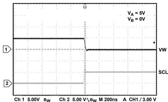
Figure 27. Midscale Glitch, Code 0x80 \geq 0x7F
