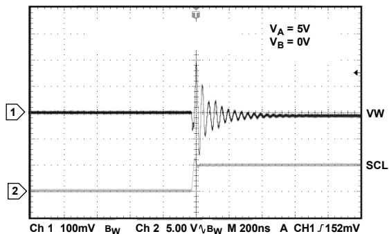
Figure 26. Digital Feedthrough
