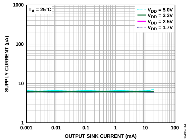
Figure 16. Supply Current vs. Output Sink Current
