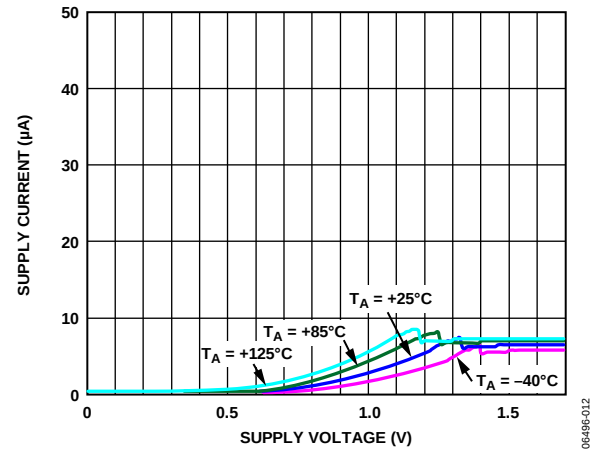
Figure 15. Start-Up Supply Current
