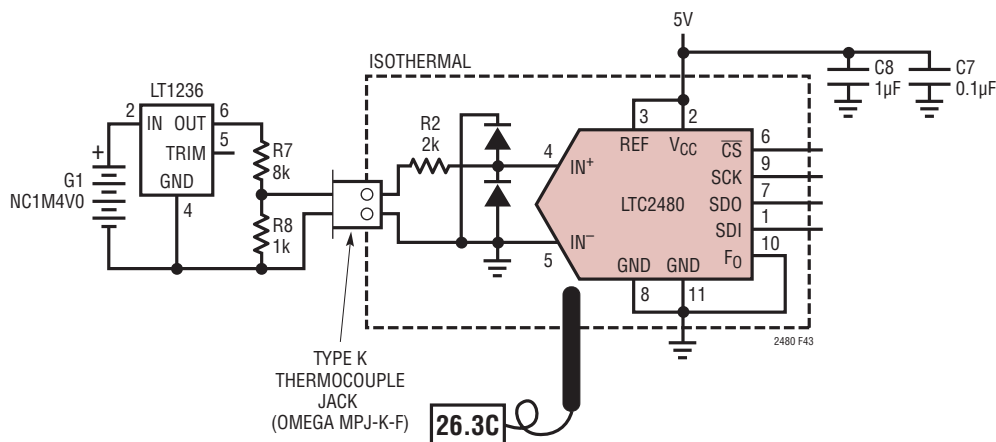
Figure 43. Calibration Setup
