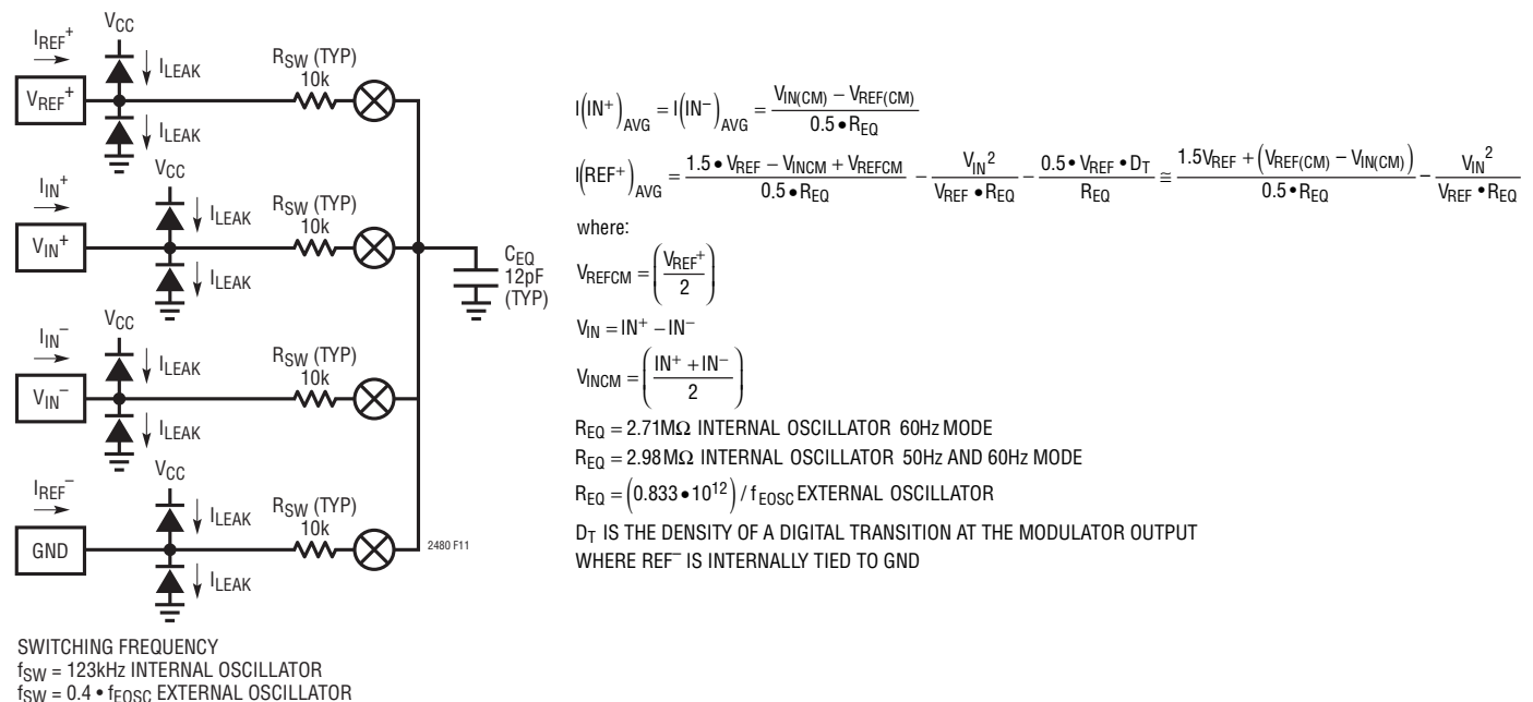
Figure 11. LTC2480 Equivalent Analog Input Circuit
