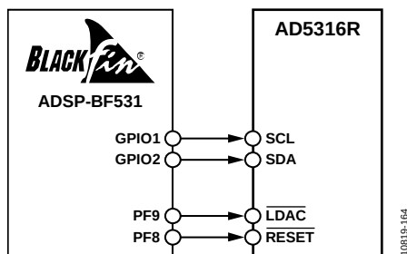
Figure 48. AD5316R to ADSP-BF531 Interface
