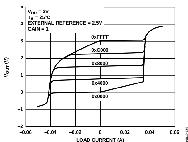
Figure 27. Source and Sink Capability at 3 V
