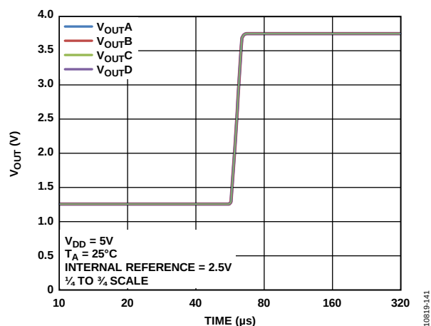
Figure 29. Settling Time
