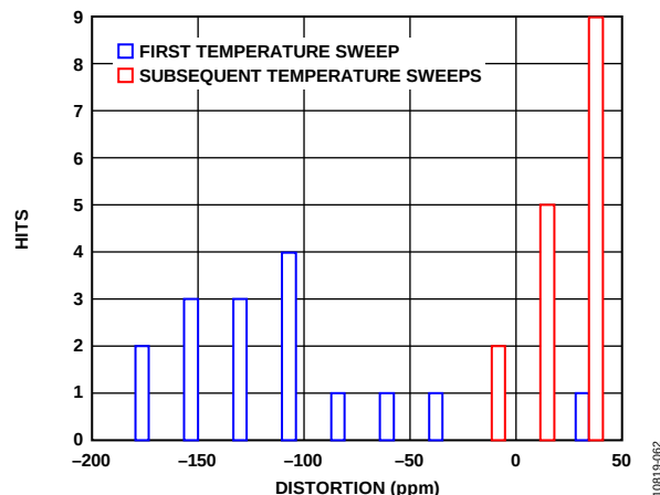
Figure 47. Thermal Hysteresis
