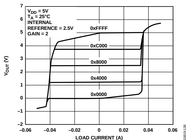
Figure 26. Source and Sink Capability at 5 V
