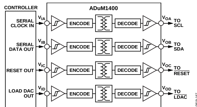
Figure 50. Isolated Interface
