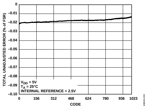
Figure 22. TUE vs. Code
