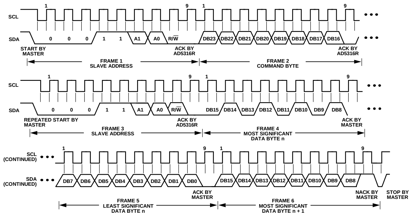
Figure 43. I²C Read Operation
