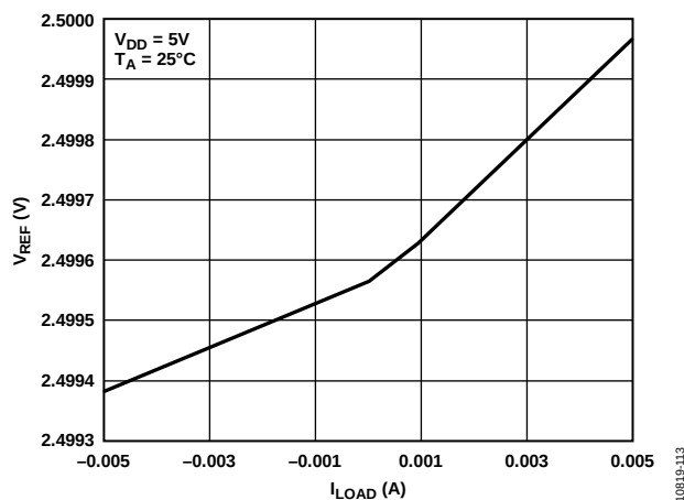
Figure 9. Internal Reference Voltage vs. Load Current
