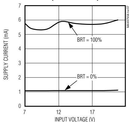
SUPPLY CURRENT vs. INPUT VOLTAGE (DPWM DIMMING)
