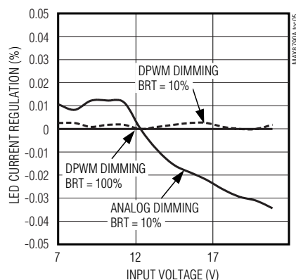
LED CURRENT REGULATION vs. INPUT VOLTAGE
