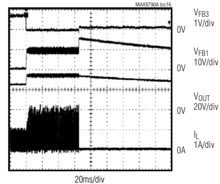
LED-OPEN FAULT PROTECTION (BRT = 100%, LED OPEN ON FB3)
