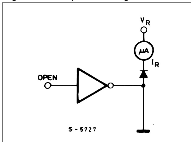
Figure 9. Clamp diode leakage current
