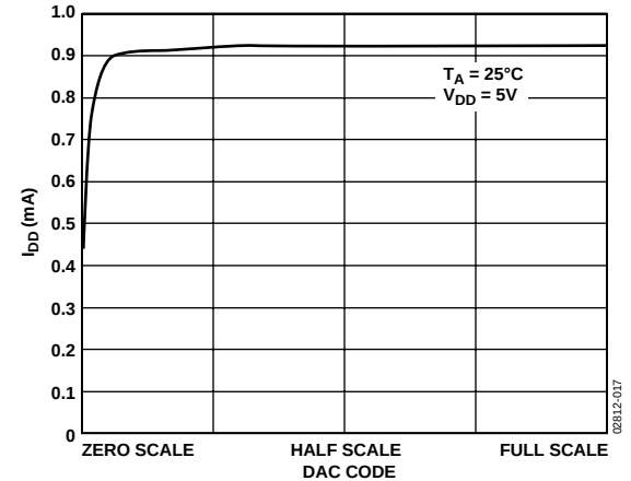
Figure 17. Supply Current vs. DAC Code
