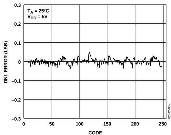
Figure 9. AD5308 Typical DNL Plot
