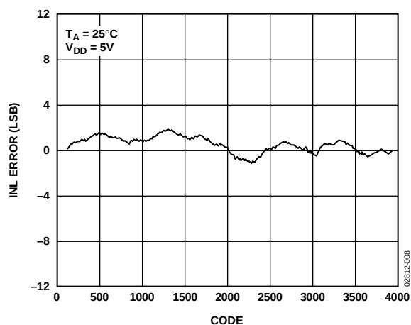
Figure 8. AD5328 Typical INL Plot
