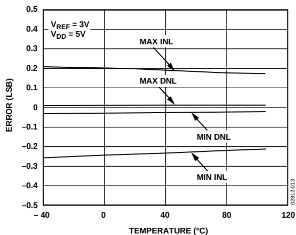
Figure 13. AD5308 INL Error and DNL Error vs. Temperature
