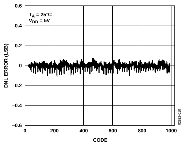
Figure 10. AD5318 Typical DNL Plot
