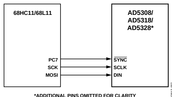
Figure 37. 68HC11/68L11 to AD5308/AD5318/AD5328 Interface
