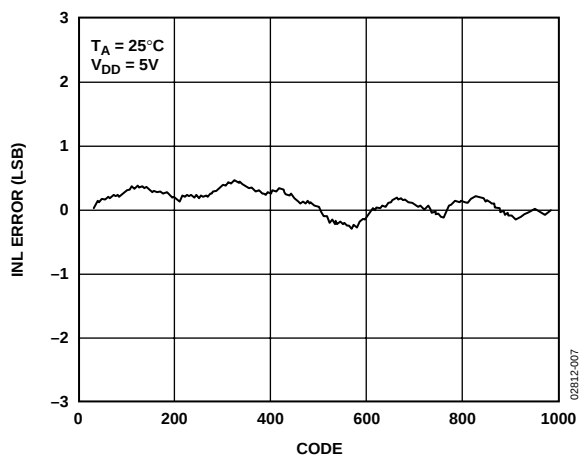
Figure 7. AD5318 Typical INL Plot
