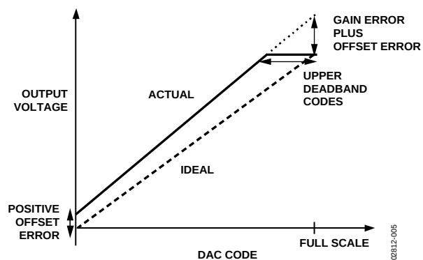
Figure 5. Transfer Function with Positive Offset
