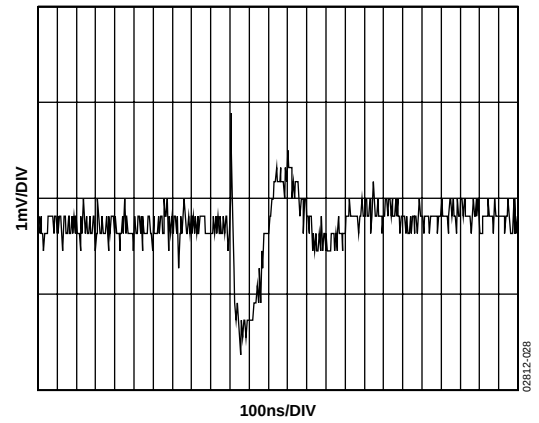
Figure 28. DAC-to-DAC Crosstalk
