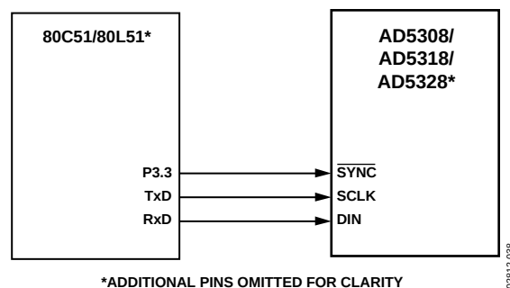
Figure 38. 80C51/80L51 to AD5308/AD5318/AD5328 Interface
