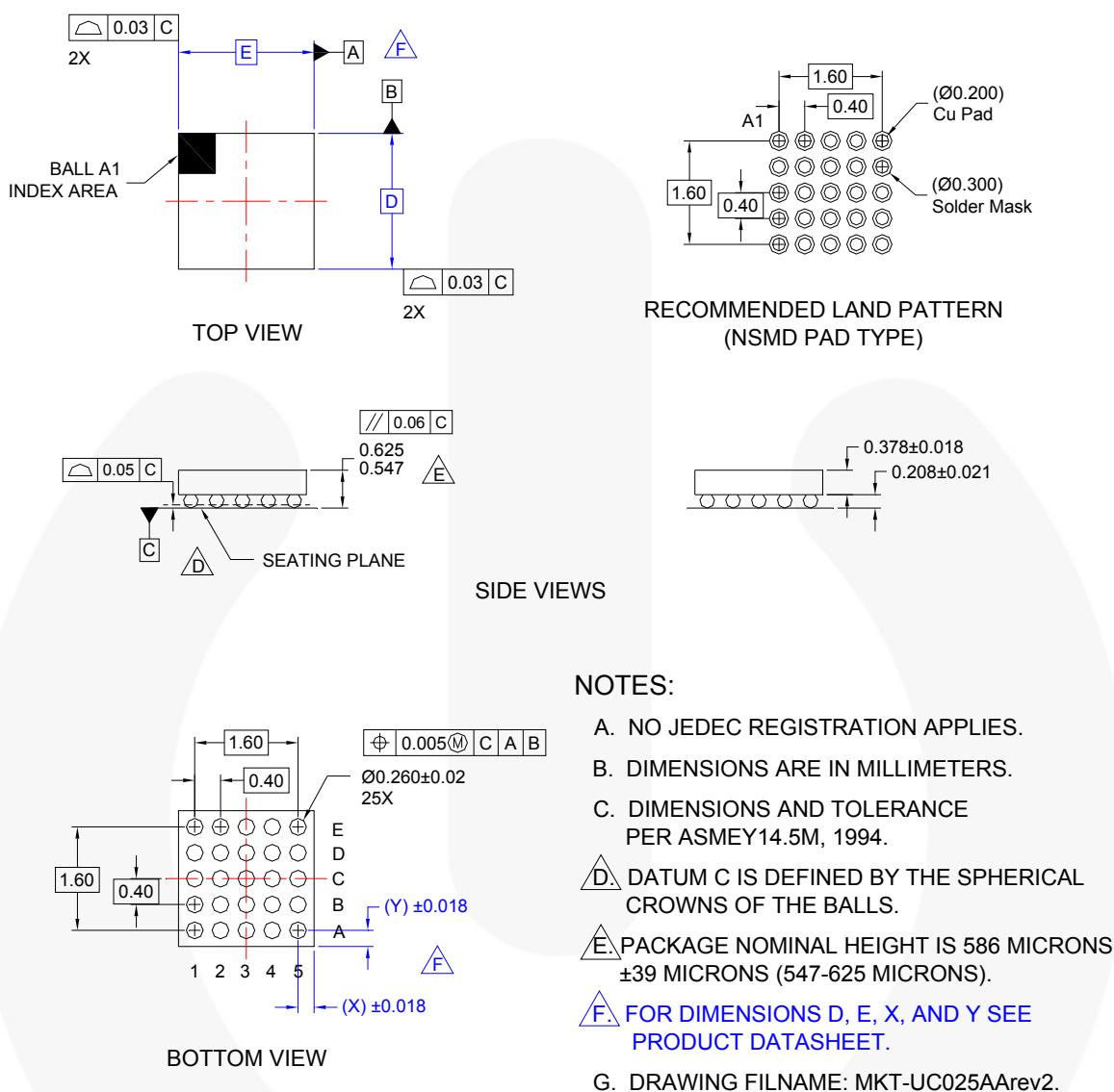
Figure 25. 25-Lead, Wafer-Level Chip-Scale Package (WLCSP)
