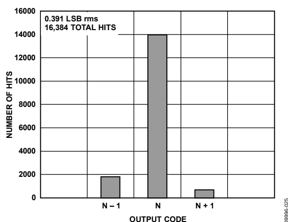
Figure 27. AD9634-210 Grounded Input Histogram, f_s = 210 MSPS
