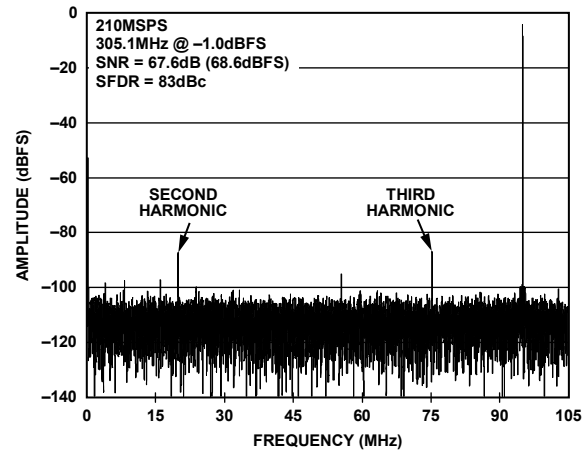
Figure 19. AD9634-210 Single-Tone FFT with f_{IN} = 305.1 MHz
