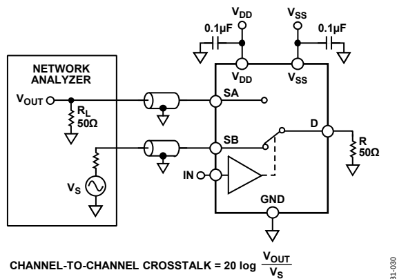
Figure 34. Channel-to-Channel Crosstalk
