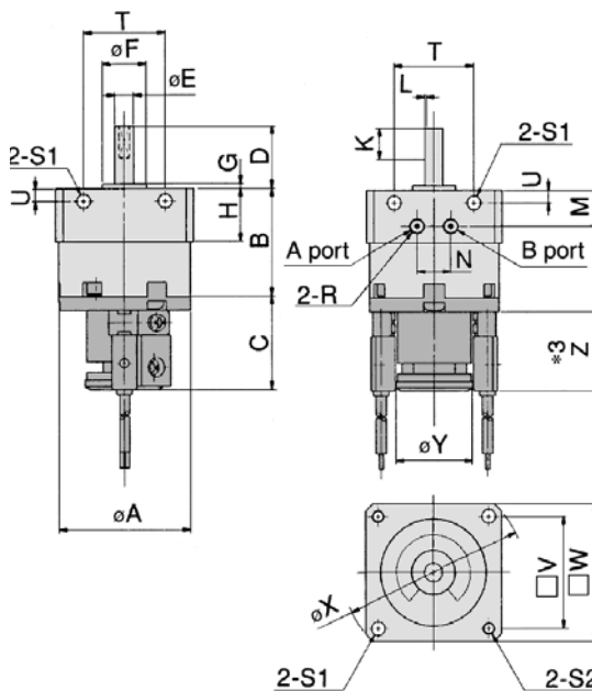
(Approx. 26.5 for connector type) CDRBU2W20, 30-□D
