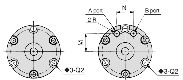
CRB2BW15, 20, 30-□DE <Port position: Axial ports>
