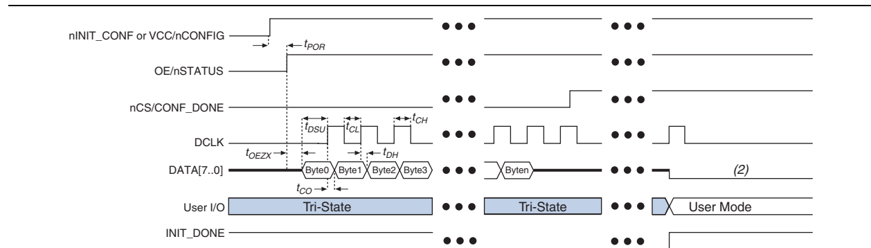
Figure 1-7. Configuration Timing Waveform Using an Enhanced Configuration Device
