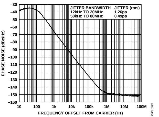
Figure 7. Phase Noise ( f_{REF} = 19.44\text{ MHz} , f_{OUT1} = 155.52\text{ MHz} )
