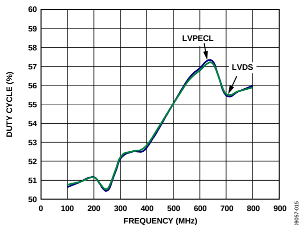
Figure 17. Duty Cycle vs. Output Frequency, LVPECL and LVDS (100 \Omega Load)
