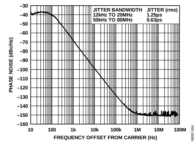
Figure 5. Phase Noise ( f_{REF} = 61.44\text{ MHz} , f_{OUT1} = 122.88\text{ MHz} )
