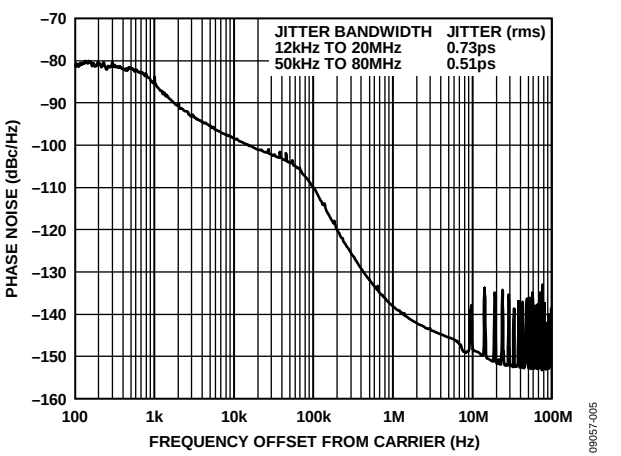
Figure 6. Phase Noise ( f_{REF} = 77.76\text{ MHz} , f_{OUT1} = 622.08\text{ MHz} )
