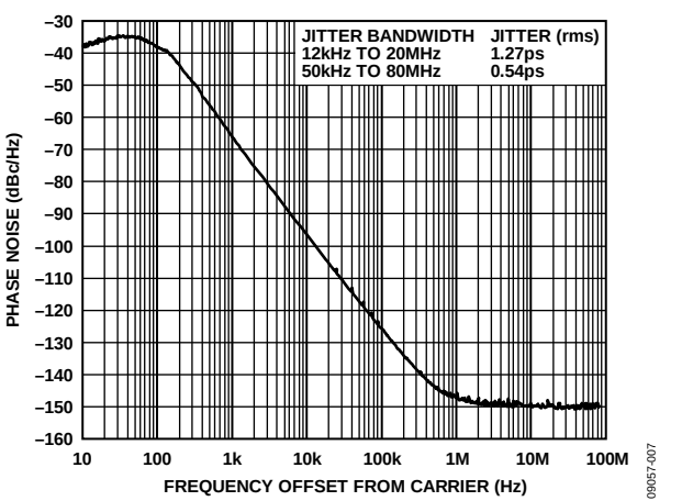
Figure 8. Phase Noise ( f_{REF} = 8\text{ kHz} , f_{OUT1} = 155.52\text{ MHz} )
