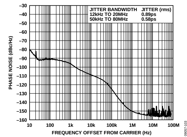
Figure 3. Phase Noise ( f_{REF} = 25\text{ MHz} , f_{OUT1} = 125\text{ MHz} )
