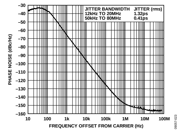
Figure 4. Phase Noise ( f_{REF} = 25\text{ MHz} , f_{OUT1} = 156.25\text{ MHz} )
