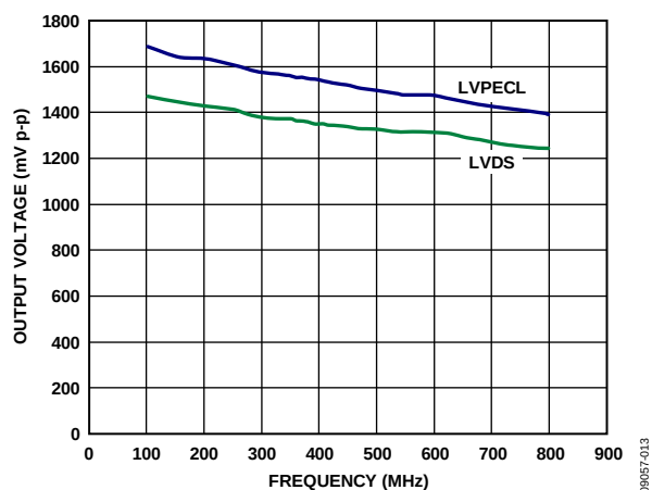
Figure 15. Peak-to-Peak Output Voltage vs. Frequency, LVPECL and LVDS (100 \Omega Load)
