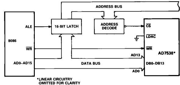
Figure 8. AD7538-8086 Interface Circuit
