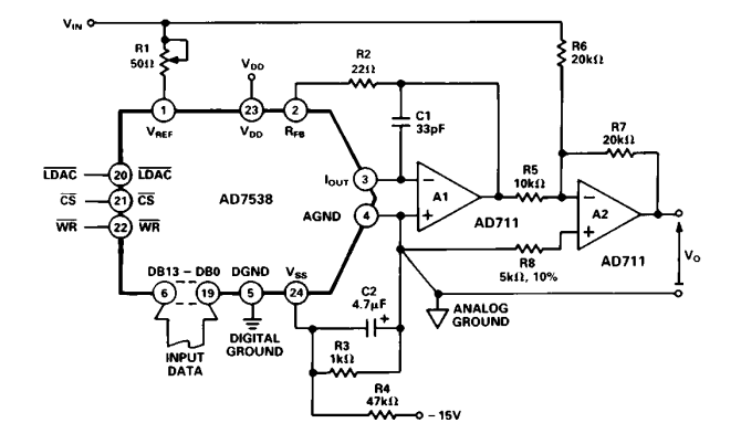
Figure 5. Bipolar Operation
