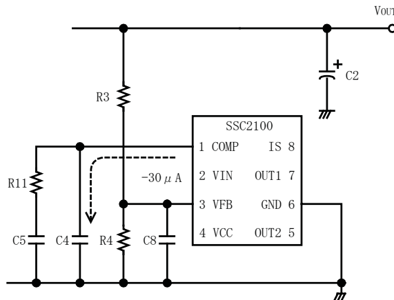
Figure 5. External circuits of VFB and COMP terminals
