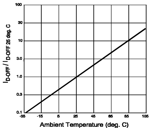
Figure 4. Typical Normalized Off-State Leakage
