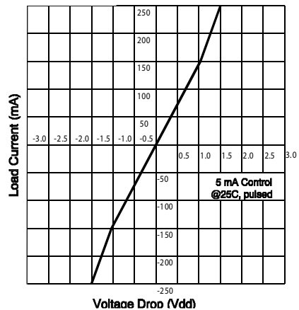
Figure 2. Linearity Characteristics
