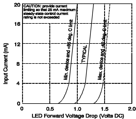
Figure 5. Input Characteristics (Current Controlled)
