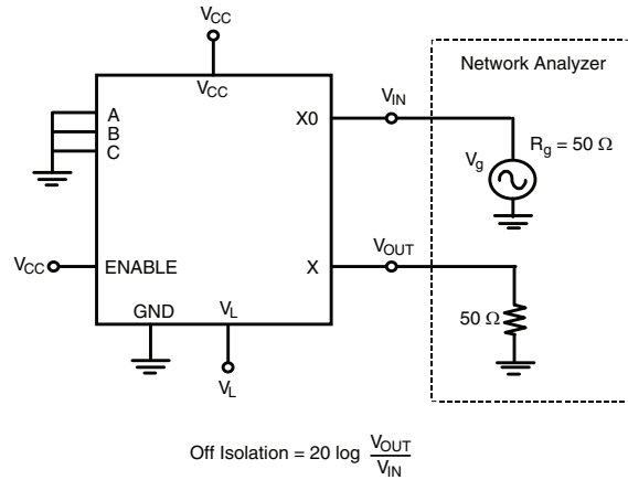
Figure 6. Off Isolation
