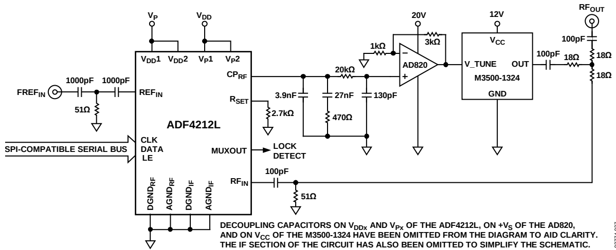
Figure 32. Wideband PLL Circuit
