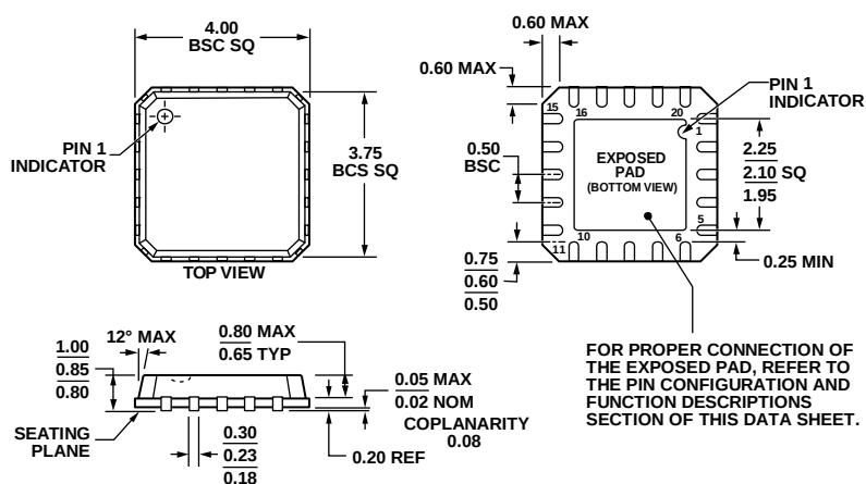
Figure 36. 20-Lead Lead Frame Chip Scale Package [LFCSP_VQ] 4 mm × 4 mm Body, Very Thin Quad (CP-20-1)
