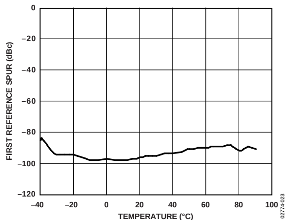
Figure 23. RF Spurs vs. Temperature
