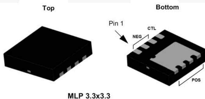
Figure 3. Pin Assignments
