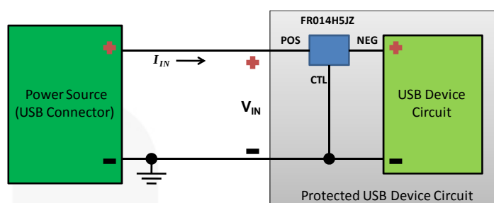
Figure 2. Typical Schematic
