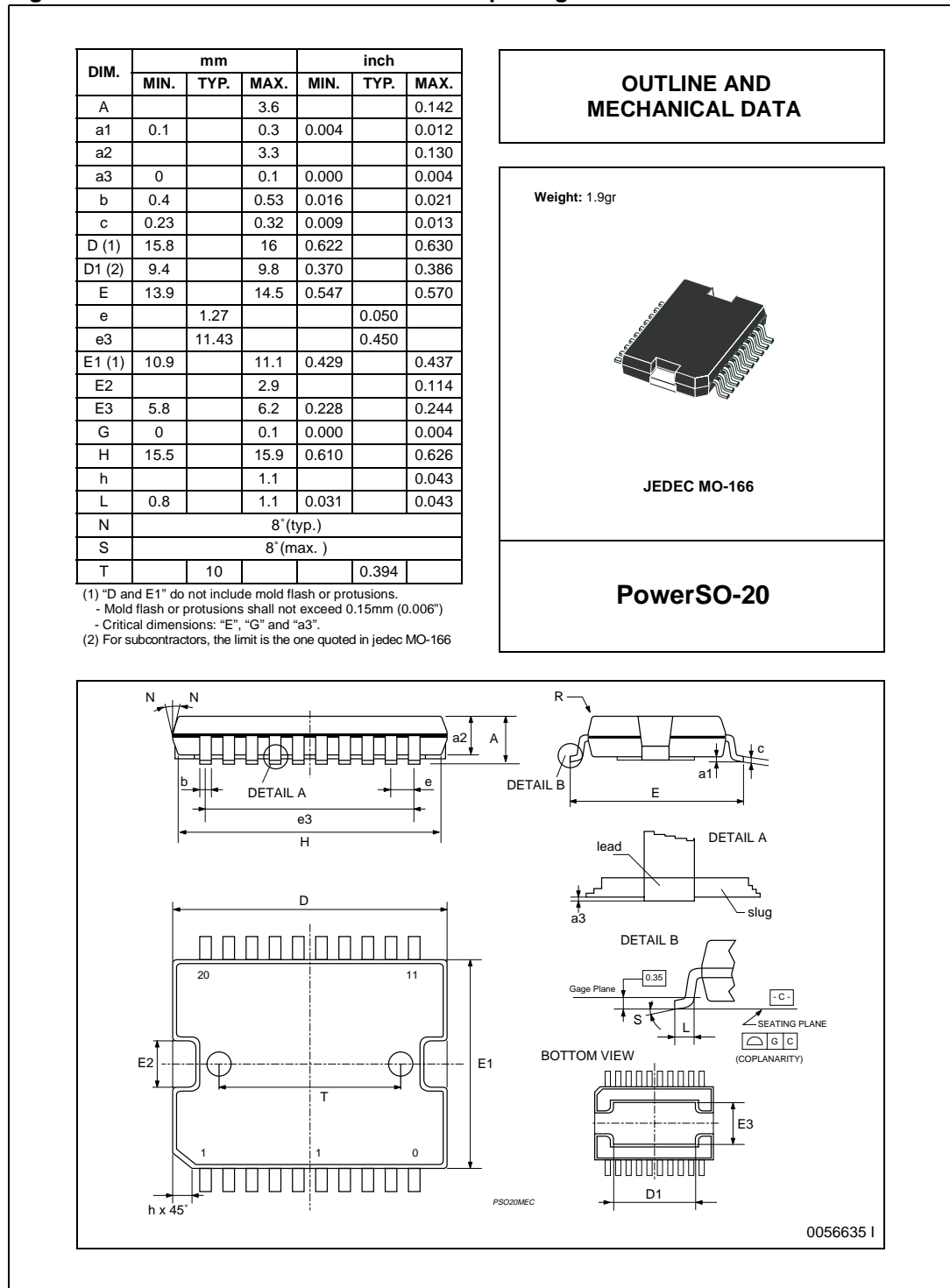
Figure 9. PowerSO-20 mechanical data & package dimensions
