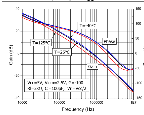
Figure 6. Voltage gain and phase vs. frequency at V_{CC} = 5\text{ V}
