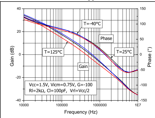
Figure 5. Voltage gain and phase vs. frequency at V_{CC} = 1.5\text{ V}
