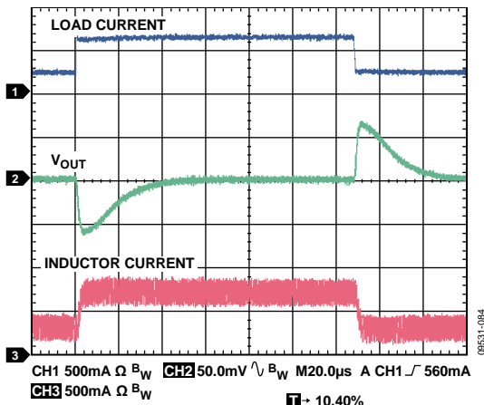
Figure 84. Output Transient Response, V_{OUT2} = 1.8\text{ V} , C_{OUT} = 10\text{ }\mu\text{F} , 300 mA to 800 mA, Load Current Rise Time = 200 ns
