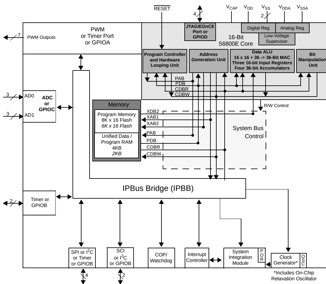
56F8013/56F8011 Block Diagram
