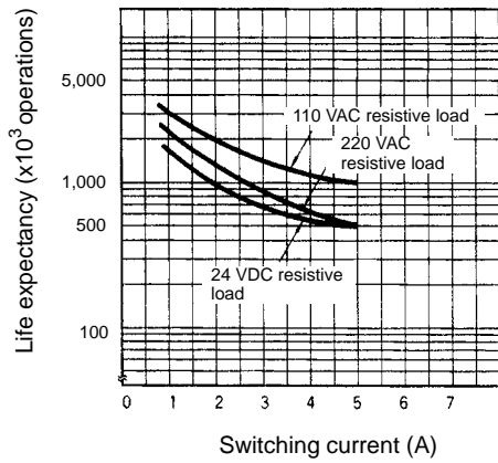
MY2-02, MY2F, MY3 Series (Resistive Loads)
