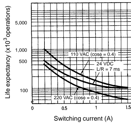
MY4Z-02, MY4ZF (Inductive Loads)
