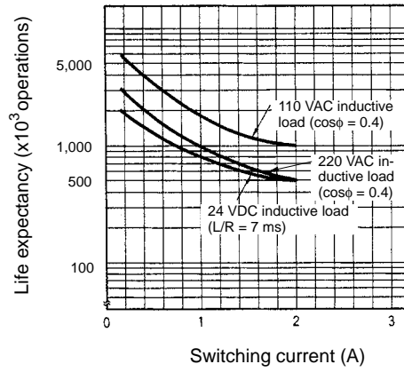
MY2-02, MY2F, MY3 Series (Inductive Loads)
