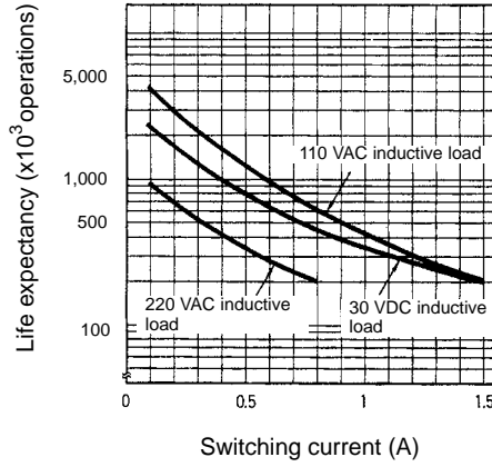
MY4-02, MY4F (Inductive Loads)
