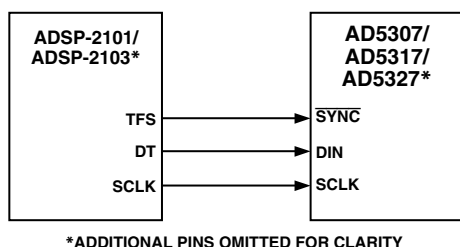
Figure 12. ADSP-2101/ADSP-2103 to AD5307/AD5317/AD5327 Interface
