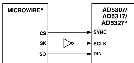
Figure 15. MICROWIRE to AD5307/AD5317/AD5327 Interface
