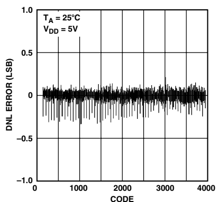
TPC 6. AD5327 Typical DNL Plot
