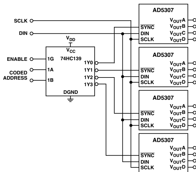
Figure 19. Decoding Multiple AD5307 Devices in a System
