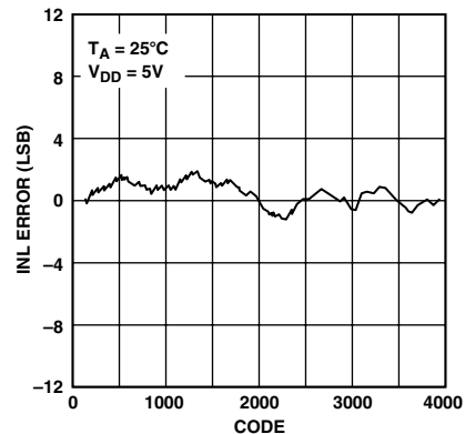
TPC 3. AD5327 Typical INL Plot
