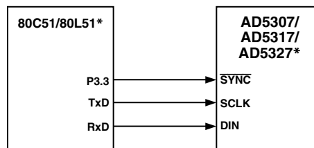
Figure 14. 80C51/80L51 to AD5307/AD5317/AD5327 Interface
