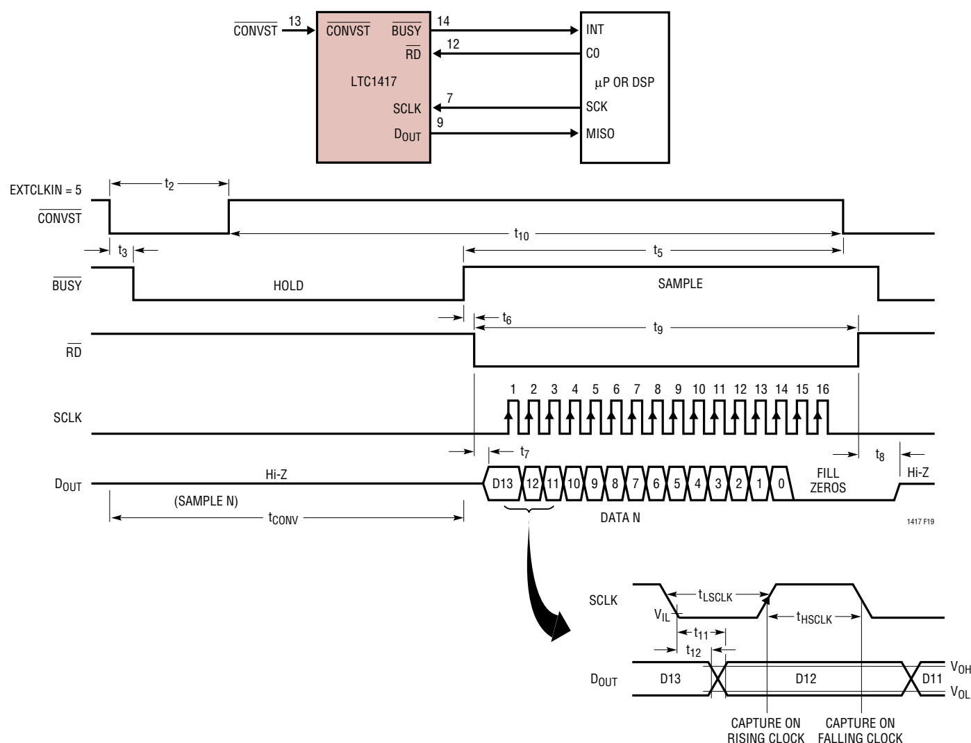
Figure 19. Internal Conversion Clock Selected. Data Transferred After Conversion Using an External SCLK. BUSY \uparrow Indicates End of Conversion
