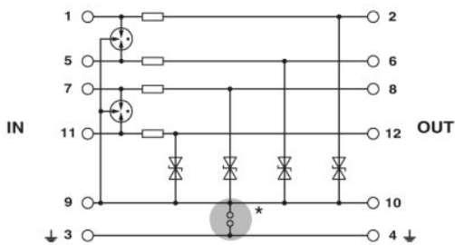
Circuit diagram
