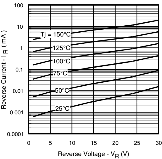
Fig. 13 - Typical Values of Reverse Current Vs. Reverse Voltage
