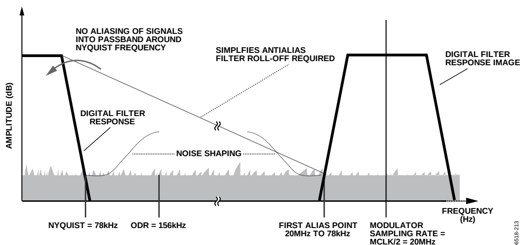
Figure 33. Antialias Example Using the AD7764 in Normal Mode, Decimate \times 128 Using MCLK/2 = ICLK = 20\text{ MHz}
