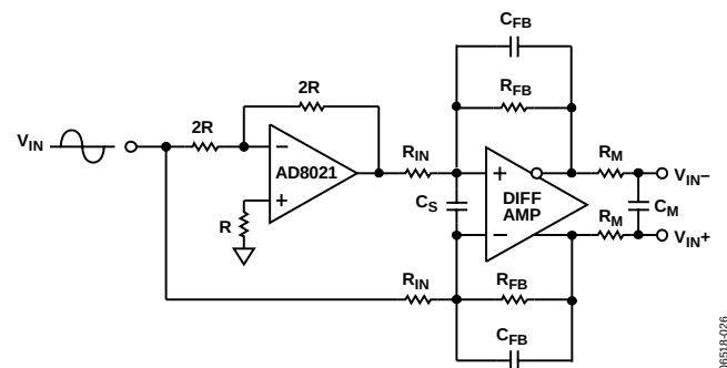
Figure 37. Single-Ended-to-Differential Conversion
