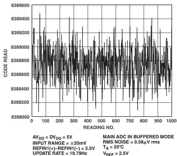
TPC 1. Typical Noise Plot on \pm 20\text{ mV} Input Range with 19.79 Hz Update Rate
