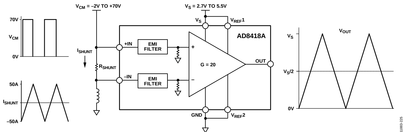
Figure 26. Typical Application
