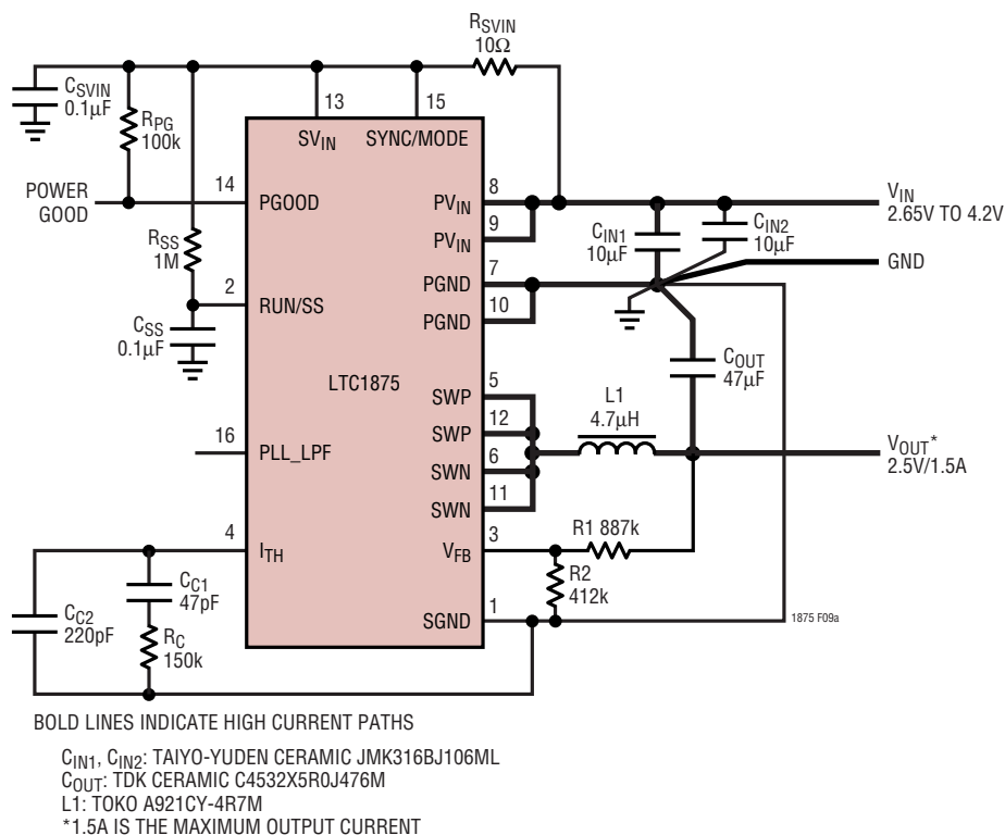
Figure 9a. Single Lithium-Ion to 2.5V/1.5A Regulator from Design Example
