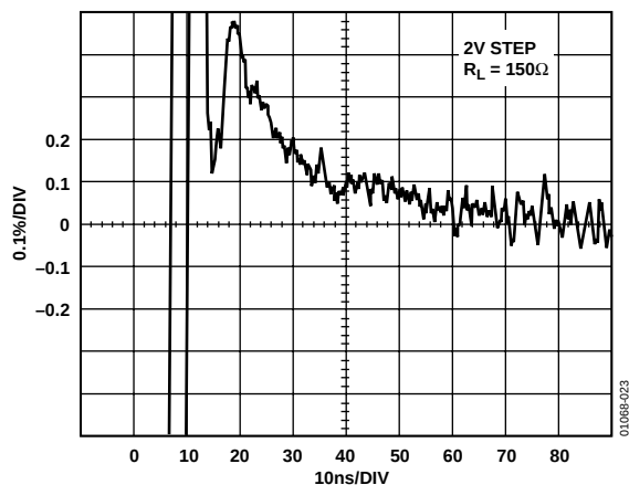
Figure 18. AD8109 Settling Time
