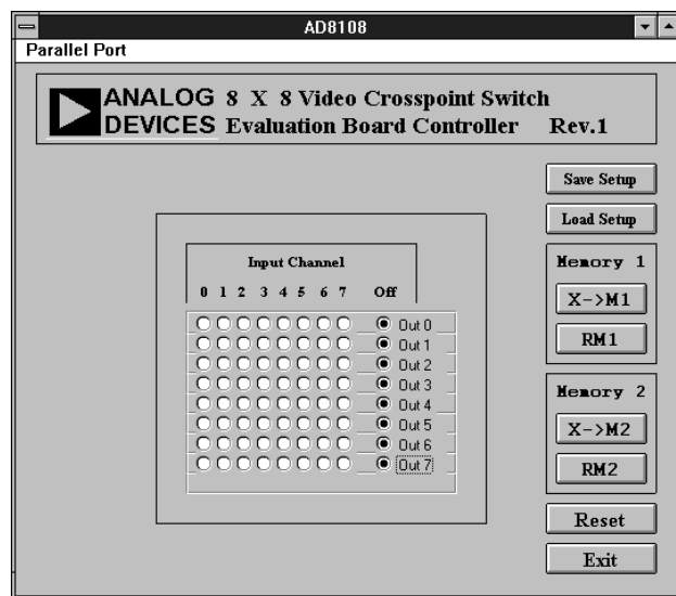
Figure 59. Evaluation Board Control Panel
