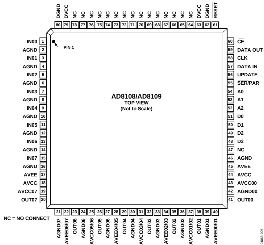
Figure 6. Pin Configuration
