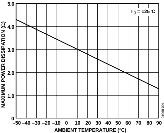
Figure 5. Maximum Power Dissipation vs. Temperature
