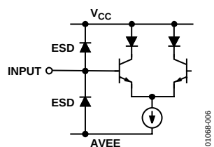
Figure 43. Analog Input
