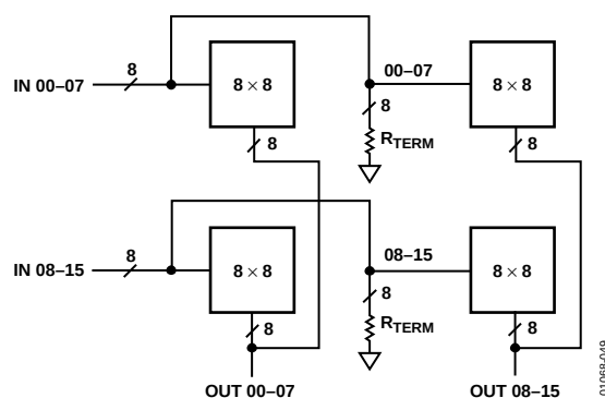
Figure 49. 16 \times 16 Crosspoint Array Using Four AD8108s or AD8109s
