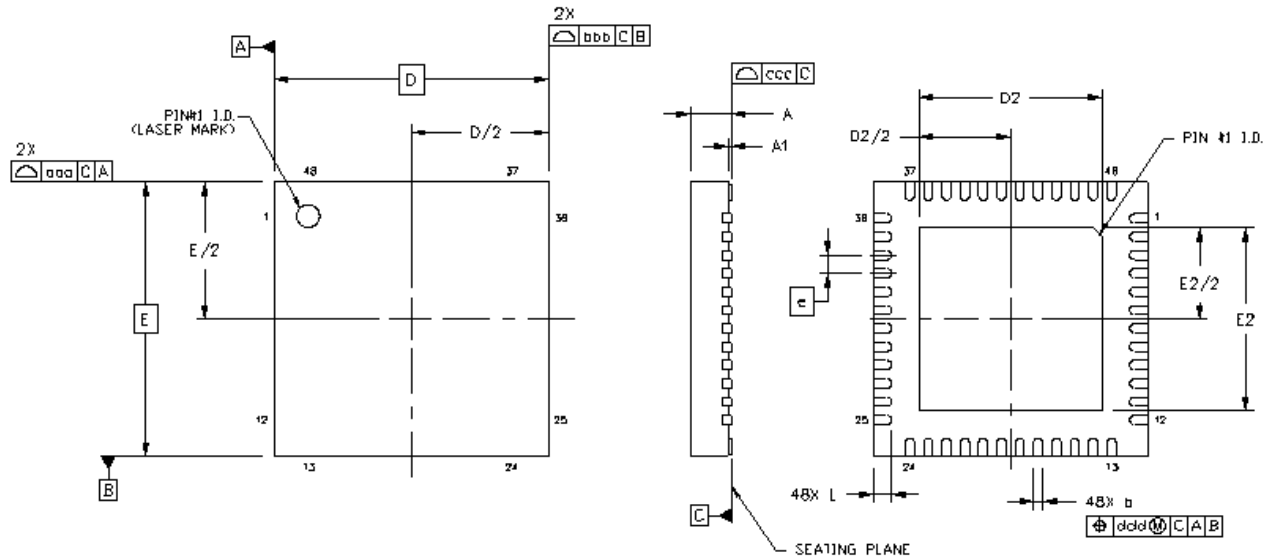
Figure 13. 72-Pin Quad Flat No Lead (QFN) Package
