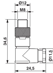
Dimensioned drawing
