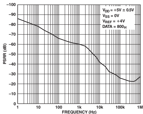
TPC 19. AD5582 PSRR vs. Frequency
