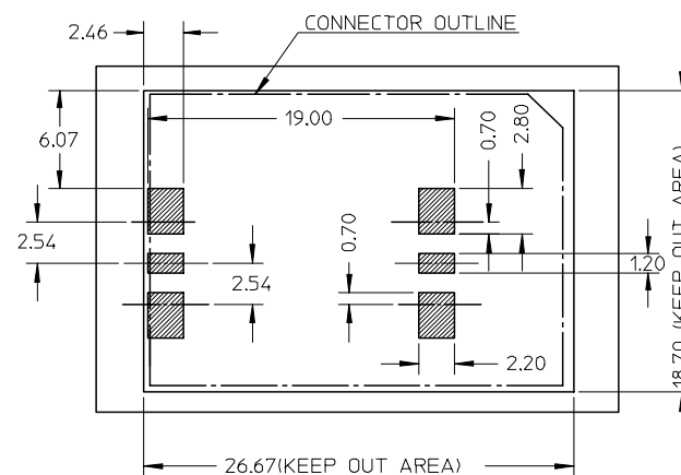
RECOMMENDED PCB LAYOUT( \pm 0.05\text{MM} )
