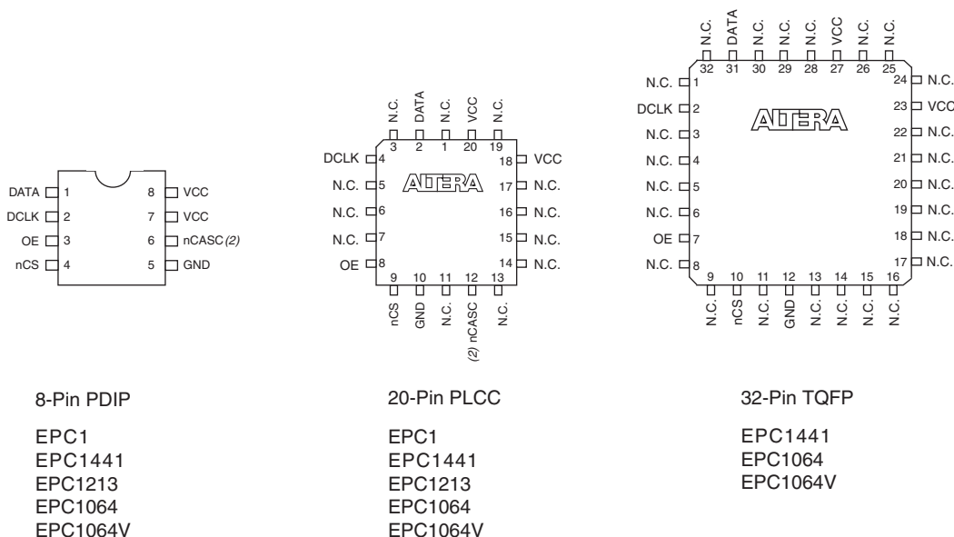
Figure 1. EPC1, EPC1441, EPC1213, EPC1064, & EPC1064V Package Pin-Out Diagrams Note (1)
